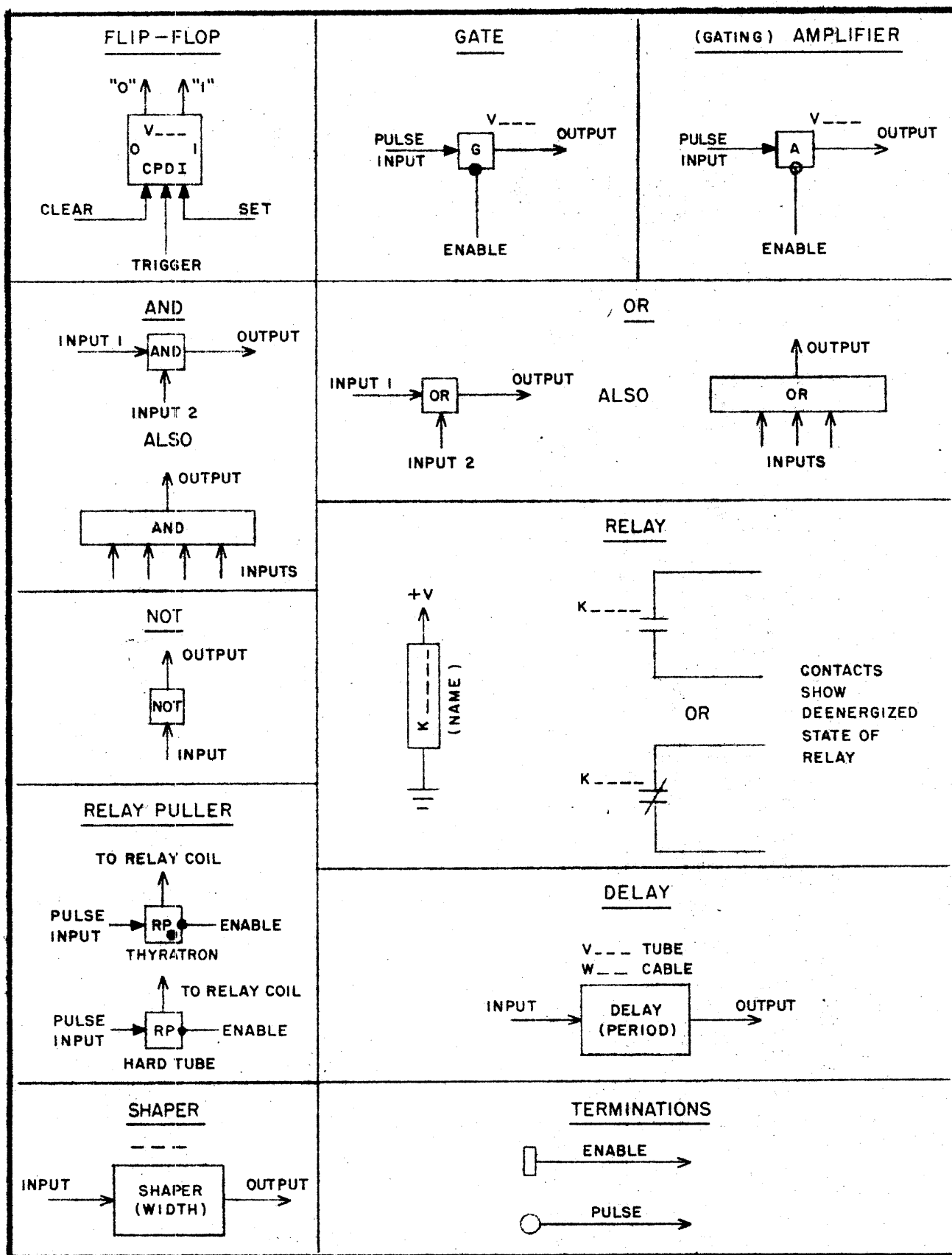
Figure 4-9. Block Symbols.
