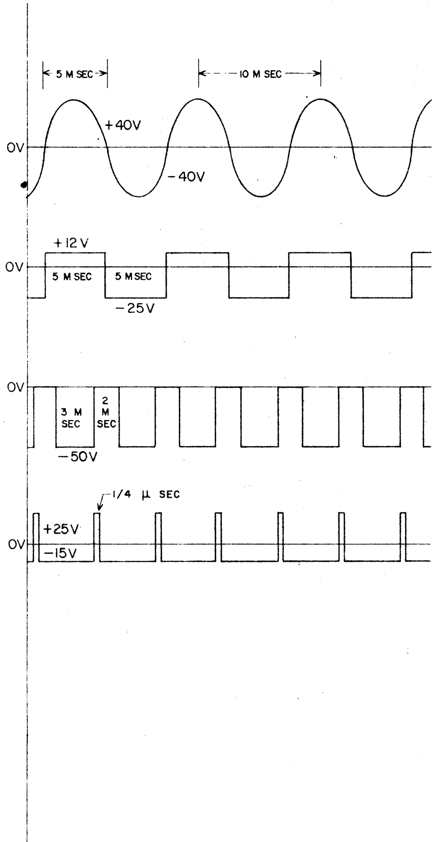
Figure 4-19. Voltage Wave forms from Ferranti Reader And Associated Circuits.
