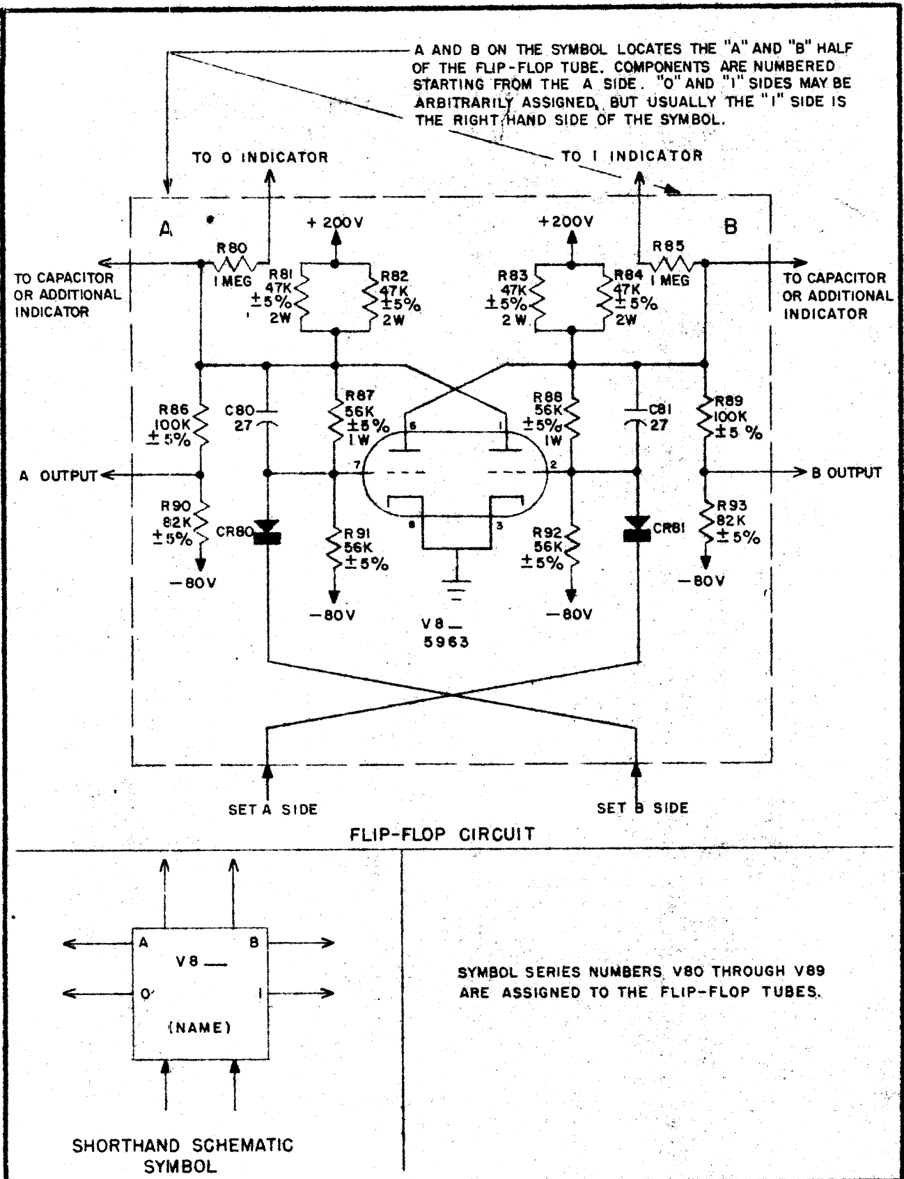
Figure 4-2. STANDARD flip-flop Stage.
