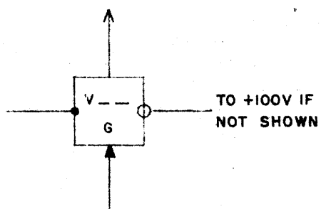
SHORTHAND SCHEMATIC SYMBOL
