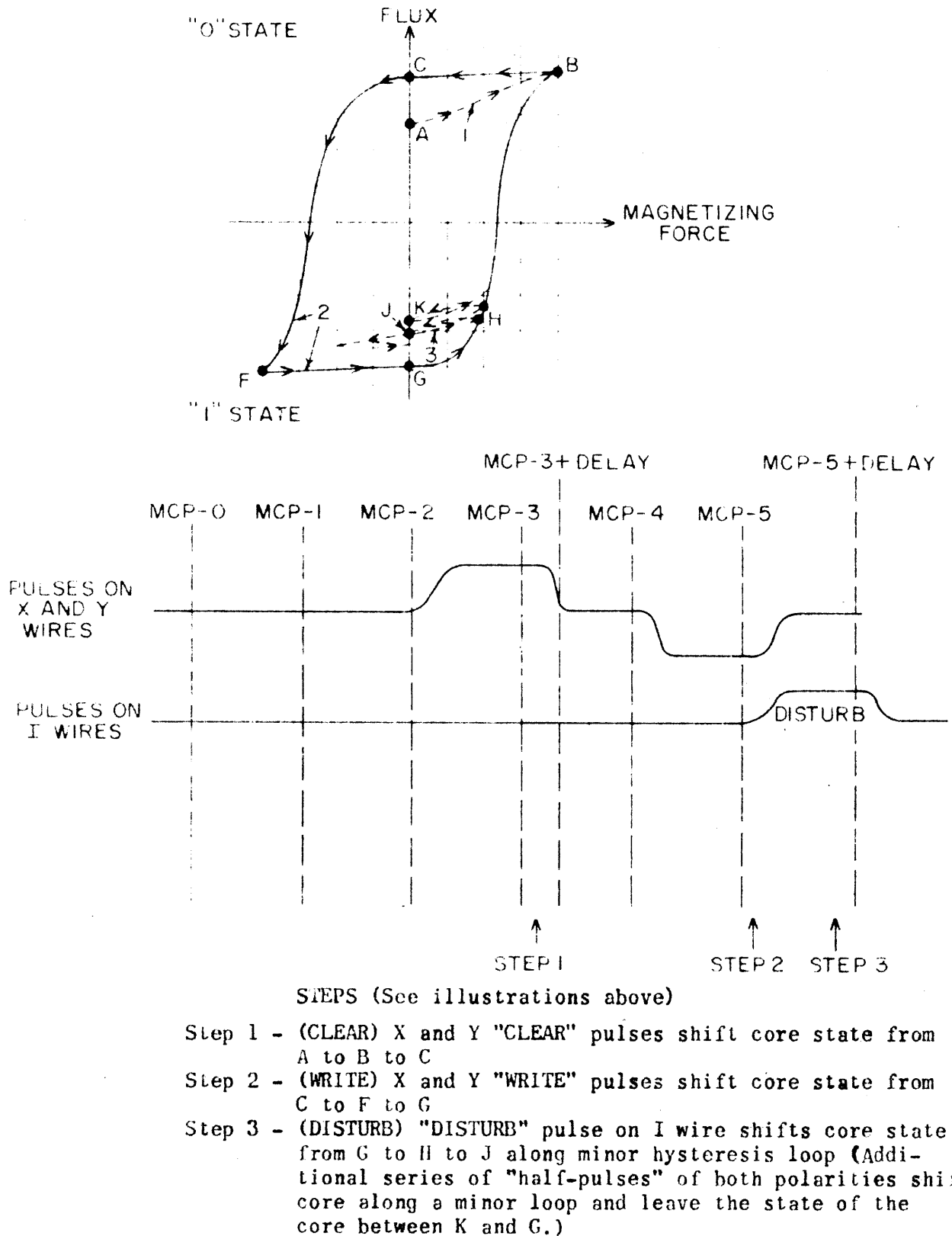
Figure 4-14. Writing a "1" When The Core Was In The "0" State
