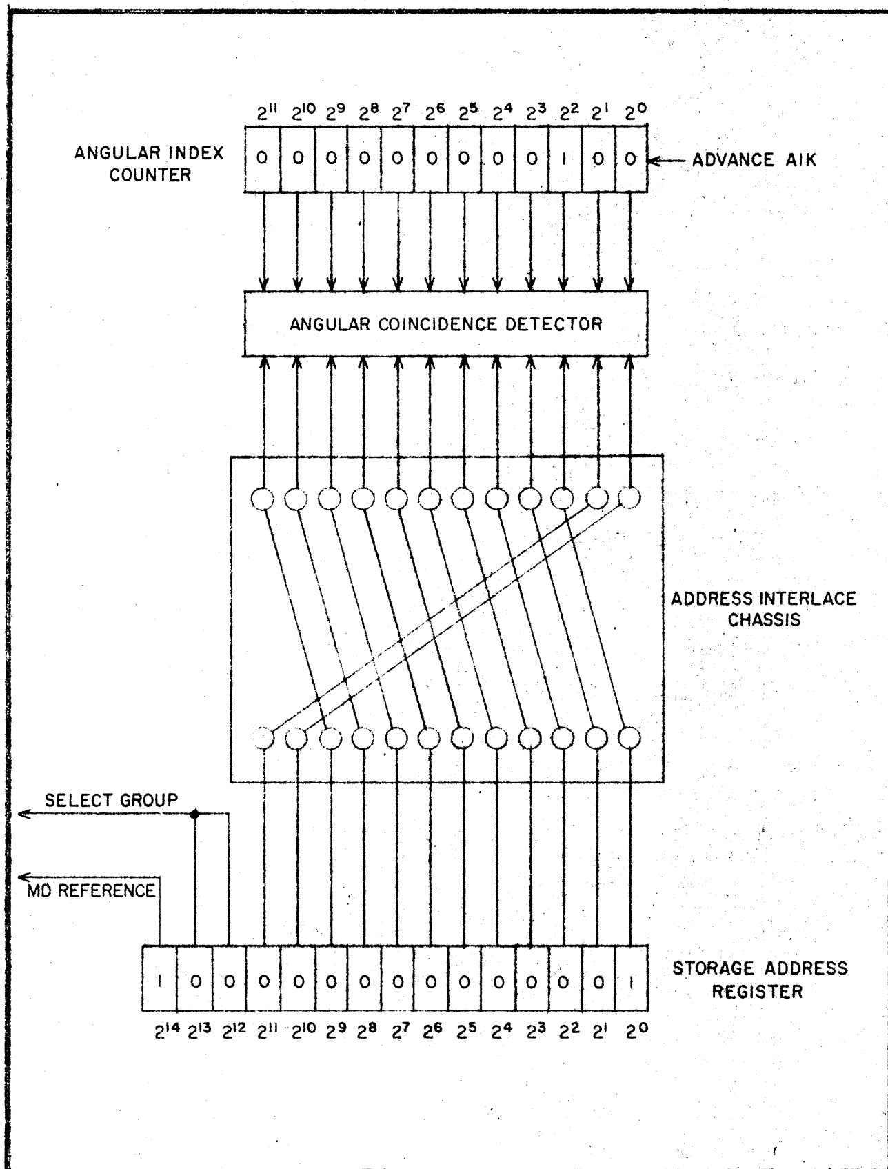
Figure 4-11. MD Locating Circuits
